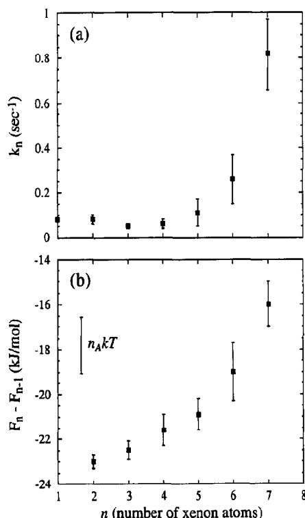
Fig. 3. (a) Xenon transfer rate coefficients, k_n , and (b) separation energies \Delta F_n , plotted as a function of xenon \alpha -cage occupancy, n . The data were determined from room temperature ^{129}\text{Xe} 2D NMR spectra acquired at 9.4 T using the sample prepared at 523 K and 30 atm xenon pressure. The constant \Delta F_1 is set to -23 kJ/mol [20].
