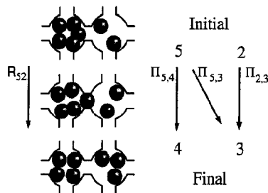
Fig. 2. Schematic representation of the relationship between the mass transport rate, R_{5,2} and the magnetization transport rates \Pi_{5,4} , \Pi_{5,3} , and \Pi_{2,3} for a single xenon intercage exchange event between Na-A \alpha -cages containing 2 and 5 xenon atoms initially. Because the ^{129}\text{Xe} NMR resonance frequency of a xenon atom occluded in Na-A zeolite depends on the number of xenon in the same \alpha -cages, three cross peaks potentially result for each intercage xenon exchange event: (1) from the active xenon atom that changes cage, (2) from the passive xenon remaining in the cage that has lost the active xenon atom, and (3) from the passive xenon in the cage that gains the active xenon atom. The magnetization transport rates are weighted by the number of xenon atoms that experience the change. Hence, for the example schematically represented the contributions to the exchange matrix are \Pi_{5,4} = 2\Pi_{2,3} = 4\Pi_{5,3} .
